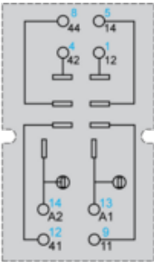
Symbols shown in blue correspond to Nema marking.
